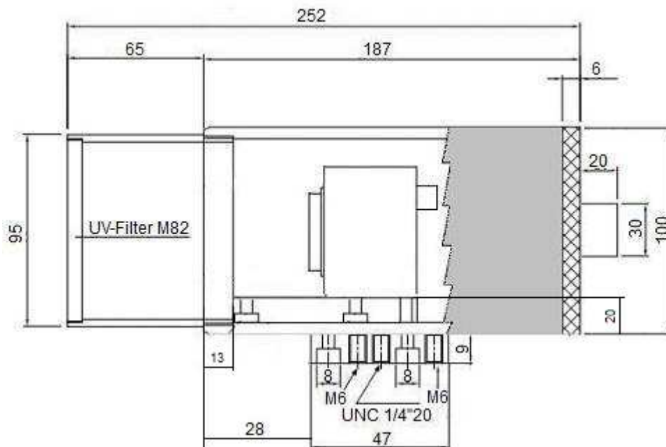
Kameraposition F-Mount
