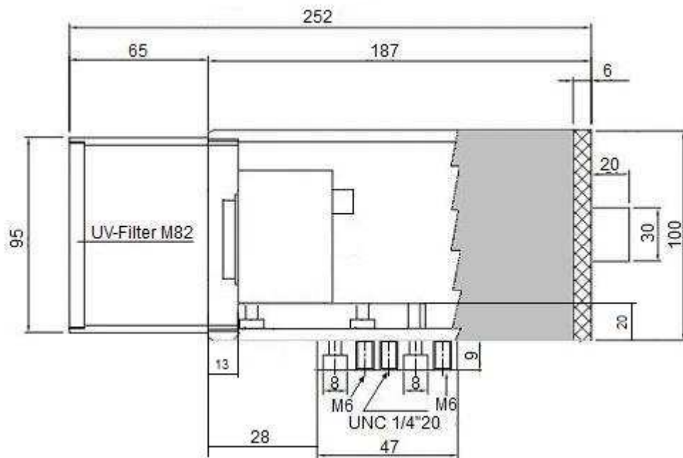
Kameraposition C-Mount
